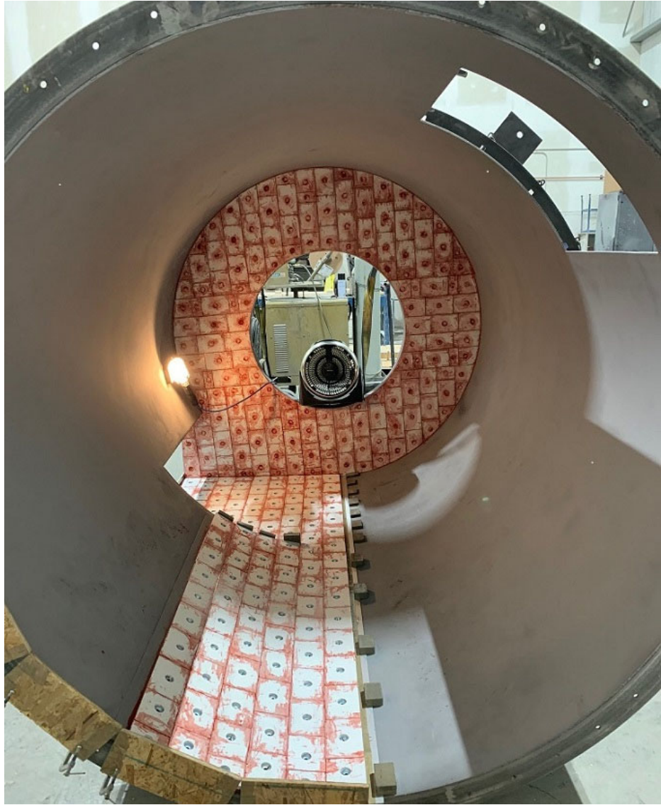
Weldable tiles being installed
